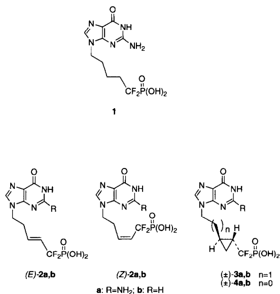
Figure 2. Novel nucleotide analogues for PNP inhibitors.
