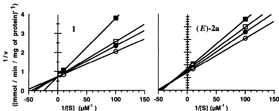
Figure 3. Lineweaver–Burk plots for inhibition of Cellulomonas sp. PNP activity by compound 1 or ( E )- 2a . Inhibitor concentration: ○, 0 μM; ●, 0.01 μM; □, 0.1 μM; △, 0.5 μM; ■, 1.0 μM.
