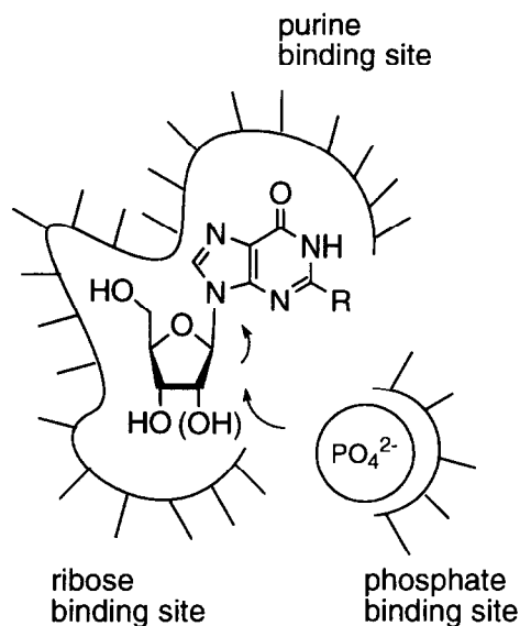
Figure 1. Schematic drawing of ternary complex of PNP and substrates.
